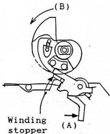
[Figure 1] Winding unit rear view
