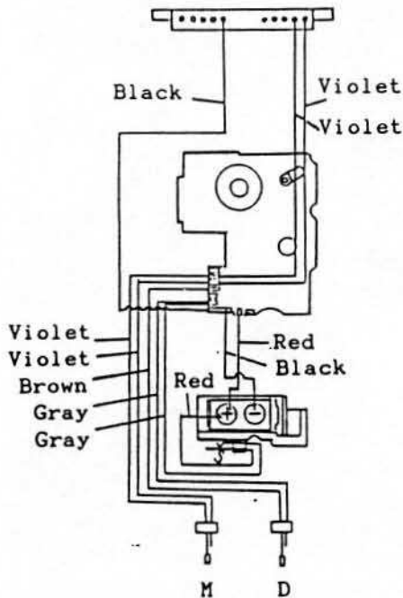
AE connector
