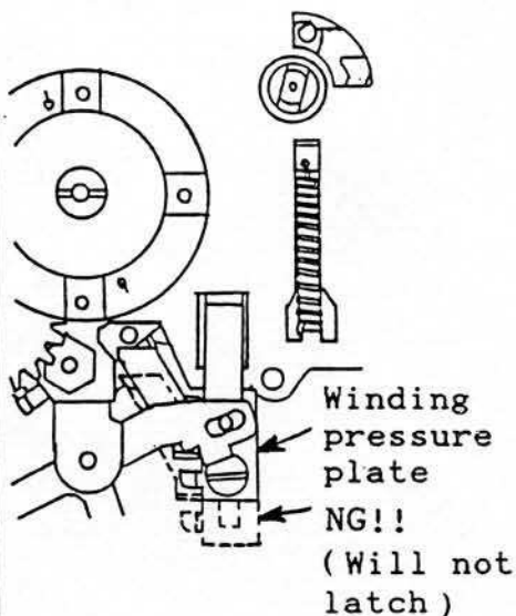
[Figure 2] Winding unit front view
